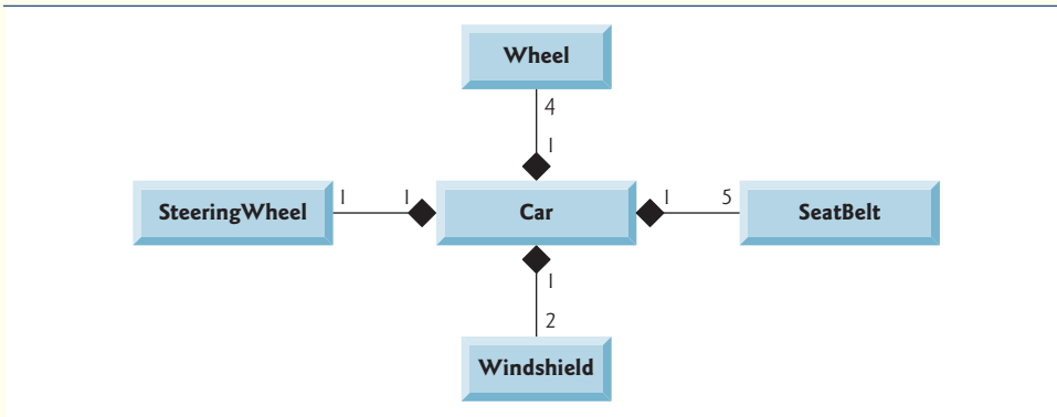
Fig. 12.27 | Class diagram showing composition relationships of a class Car.
