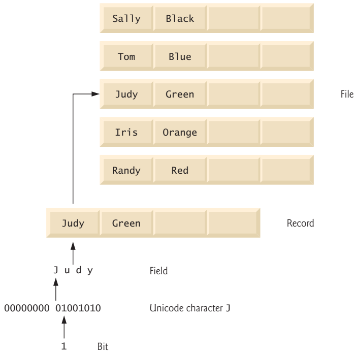
Fig. I.2 | Data hierarchy.
